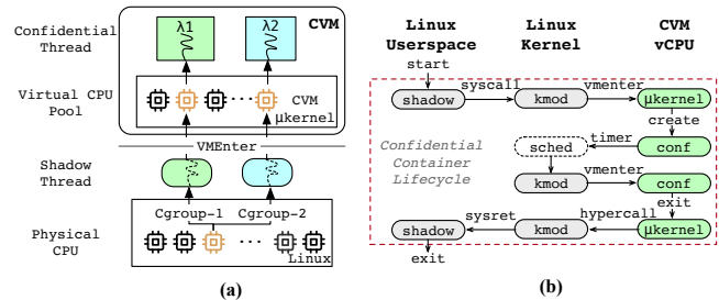
Figure 7. (a) CPU resource granting mechanism, (b) the CPU control flow of a confidential container (I/O delegation is not included for simplicity), shadow: shadow container, conf: confidential container, kmod: host module, \mu kernel: CVM microkernel.
