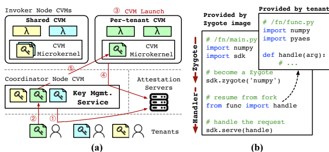
Figure 6. (a) Key dispatching, (b) A Zygote example.
