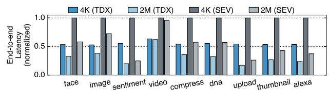
Figure 14. Effects of huge page granting optimization.
