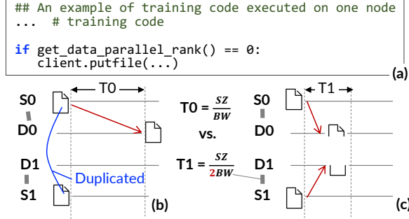
Figure 10: (a) A code snippet of user-implemented deduplicated grouped write [48], (b) the time of its execution and (c) the improved load-balanced write plan.
