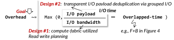
Figure 5: Design goal and how AITURBO achieves so.
