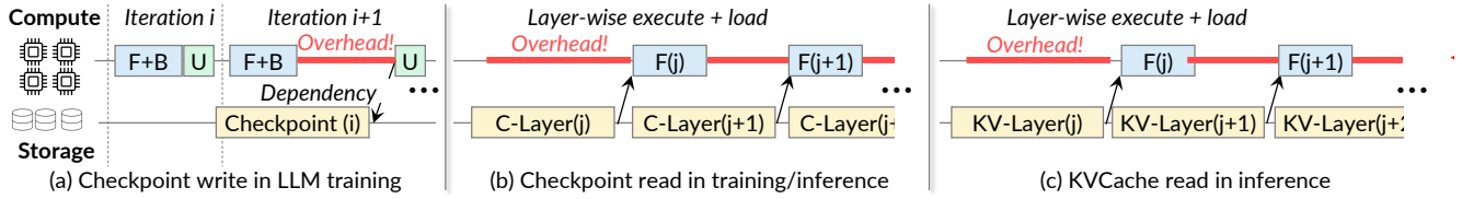
Figure 2: An illustration of how different AI jobs interact with the cloud storage as well as possible costs introduced by insufficiently fast storage I/O. F and B states abbreviate for forward and backward pass of a training job, respectively. The i in (a) indicates the i -th iteration of a training job, while the j in (b) and (c) indicates the data partitioned by the model layer, e.g., C-Layer( j ) indicates the checkpoint of the j^{\text{th}} layer.
