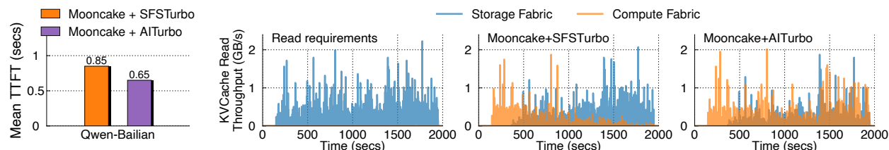
Figure 18: Evaluation results from replaying Qwen-Bailian trace [50] for 30 minutes: (a) mean time to first token (TTFT) and (b) compute/storage fabric KVCache read throughput.
