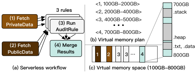
Figure 9. An illustration of generating virtual memory (VM) plan (b) given a serverless workflow (a). The plan will partition a virtual memory space for different functions (c).
