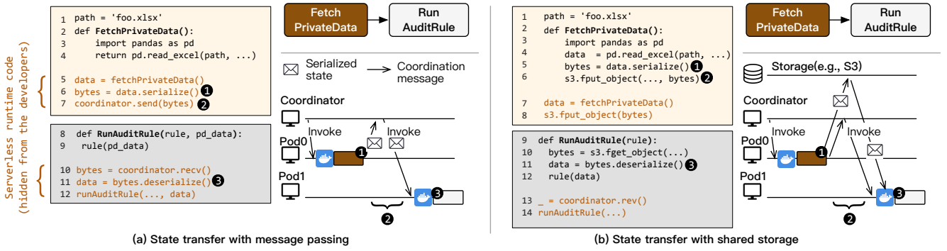
Figure 2. An overview of state transfer between two functions using (a) messaging and (b) shared storage. Functions are executed in containers at each machine (pod). The serverless runtime code will be called after receiving the coordinator message.
