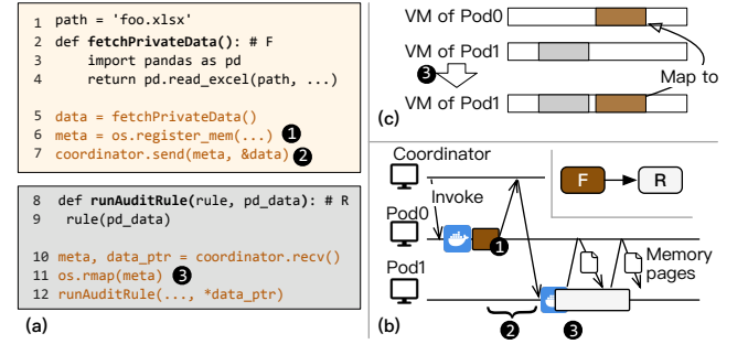
Figure 6. An overview of serverless workflow with RMMMap. (a) How serverless framework leverages RMMMap to transfer state. (b) The detailed execution flow of state transfer and (c) How pod’s virtual memory space changes with RMMMap.
