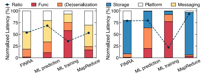
Figure 3. Analysis of the state transfer costs in representative serverless workflows: (a) using messaging and (b) shared storage. Func: function execution time, Ratio: the ratio of time of state transfer in the end-to-end time.
