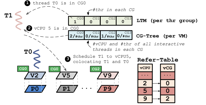
Fig. 6. The algorithm of CPS-CGsched. T0 and T1 are two interactive threads. The frontend uses LTM and CG-Tree to migrate T1 to vCPU-5, co-locating the two interactive threads.
