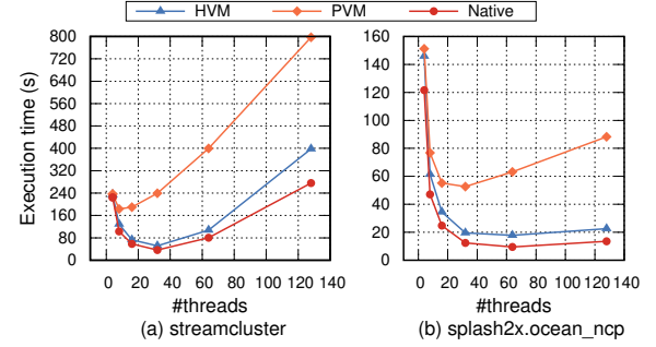
Fig. 1. Negative performance effects of the pvsched optimization.
