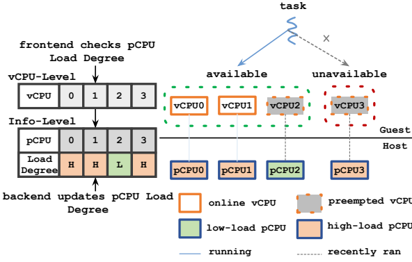
Fig. 5. The workflow of CPS-Pload. The backend updates the pCPU load degree promptly. The frontend checks pCPU loads and enlarges the available vCPU set with preempted but low-scheduling latency vCPUs (vCPU-2).
