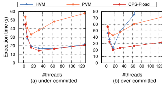
Fig. 8. The thread scalability of CPS-Pload, HVM, and PVM for splash2x.ocean_cp benchmark in the 128-vCPU VM. Lower is better.
