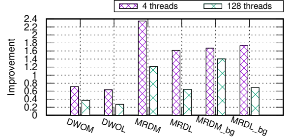
Fig. 10. The improvement of FxBench brought by CPS-CGsched in the under-committed 128-vCPU VM. Higher is better.
