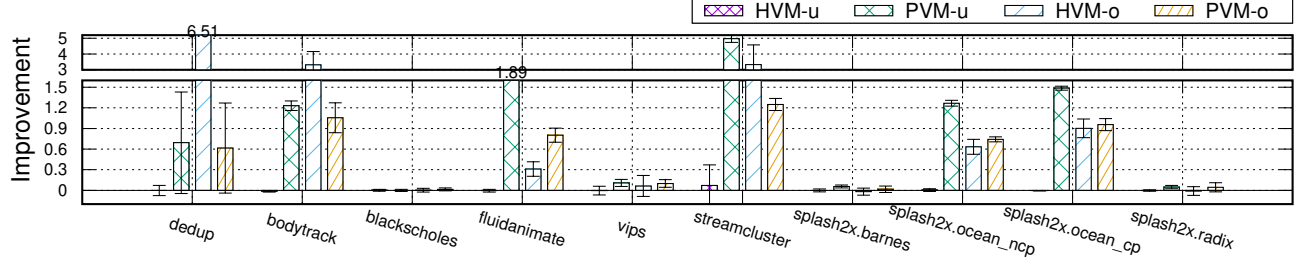
Fig. 7. Performance improvement of CPS-Pload over HVM and PVM in PARSEC 3.0 in the 32-vCPU VM. -u stands for under-committed one VM scenario and -o stands for over-committed five VMs scenario. Higher is better.
