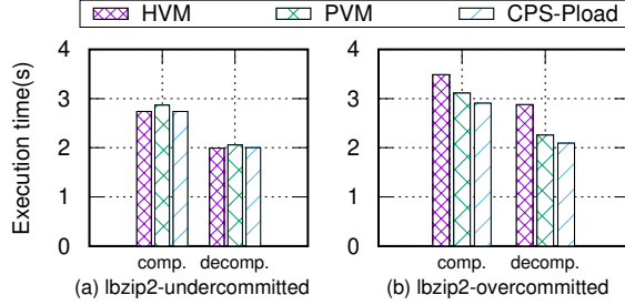
Fig. 9. The CPS-Pload improvement of lbzip2 in the 32-vCPU VM. Lower is better.
