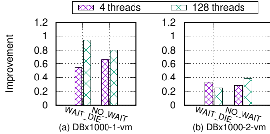
Fig. 13. The improvement of DBx1000 brought by CPS-CGsched in the 128-vCPU VM. Higher is better.
