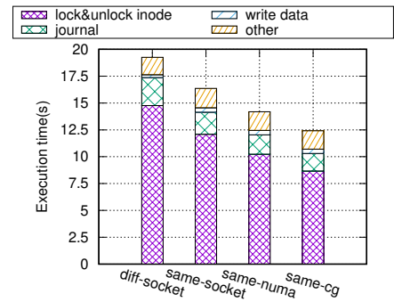
Fig. 11. The impact of memory hierarchy on the performance of DWOM in FxBench with four configurations: 1) diff-socket: 4 vCPUs are distributed in different sockets. 2) same-socket: 4 vCPUs are pinned in the same socket. 3) same-NUMA: 4 vCPUs are pinned in the same NUMA node. 4) same-CG: 4 vCPUs are pinned in the same cache group (a CG contains 4 pCPUs).
