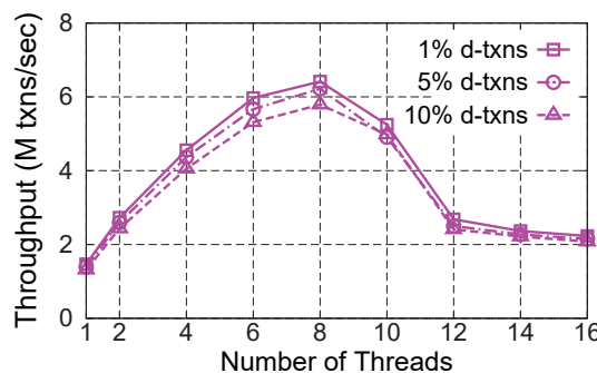
Figure 16. The throughput of standard-mix in SmallBank on DrTM+R=3 with the increase of threads using different probability of cross-machine accesses for SP and AMP .
