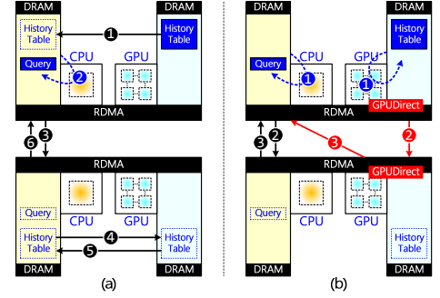
Fig. 8: Communication flow w/o and w/ GPUDirect.
