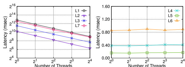
Fig. 14: The latency of queries in group (I) and (II) with the increase of threads on LUBM-10240.
