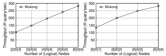
Fig. 18: The throughput of a mixture of queries with the increase of logical nodes. The tick labels of x-axis are the configuration, and the symbol of [m] \times [n] corresponds with #machines and #nodes/machine.
