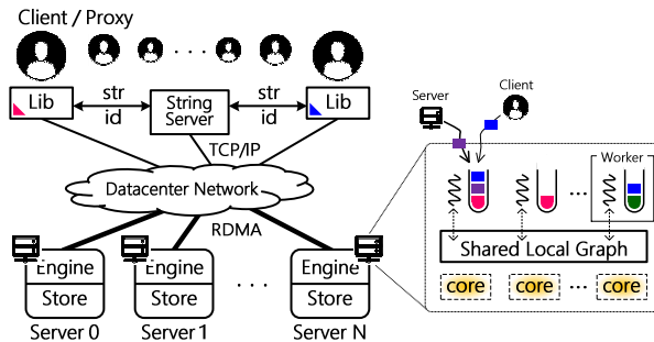
Fig. 5: The architecture overview of Wukong.
