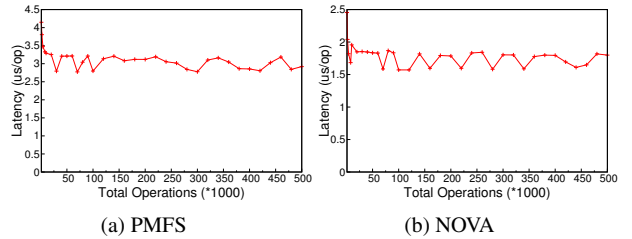
Figure 8: Append latency with deletion
