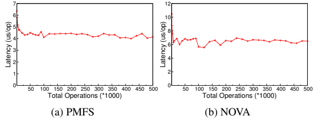
Figure 7: Latency trends with deletion
