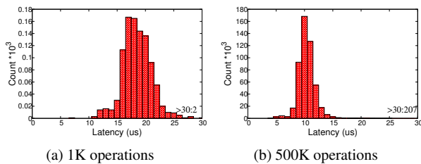
Figure 10: Latency distributions for NOVA
