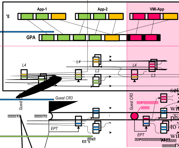
Figure 7: Memory mapping for both the implanted core and guest VM codes.
