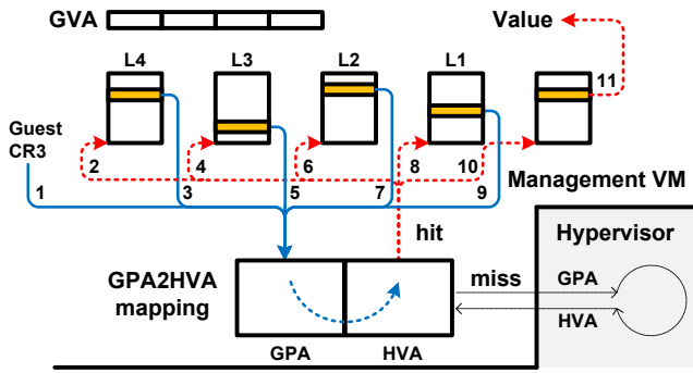
Figure 3: Software page table traversal in vmi_read_addr
