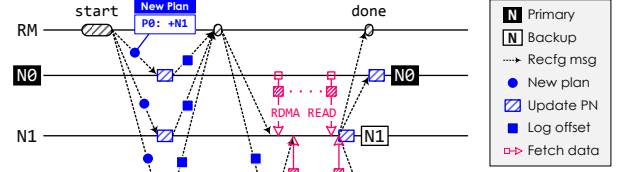
Fig. 8: The optimized execution flow of asynchronous replication. A new backup replica of P0 is created on N1.
