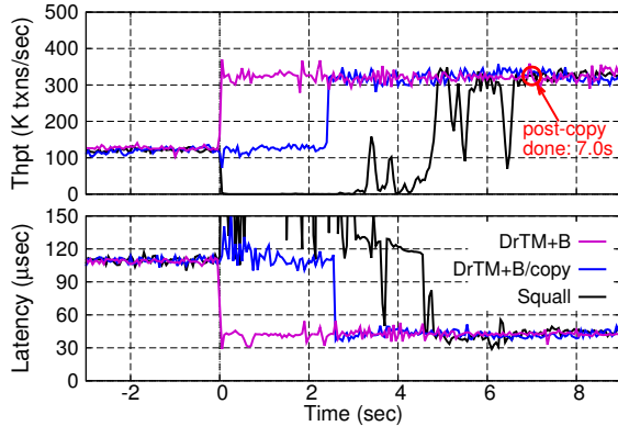
Fig. 12: The perf. timeline for TPC-C with high skew.
